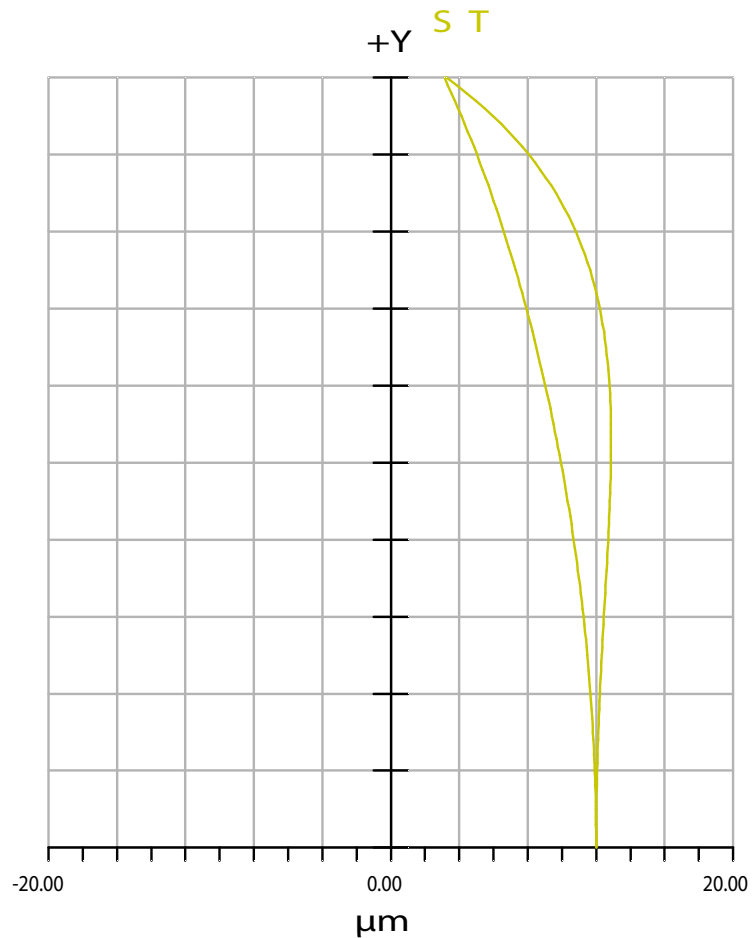
Field Curvature
