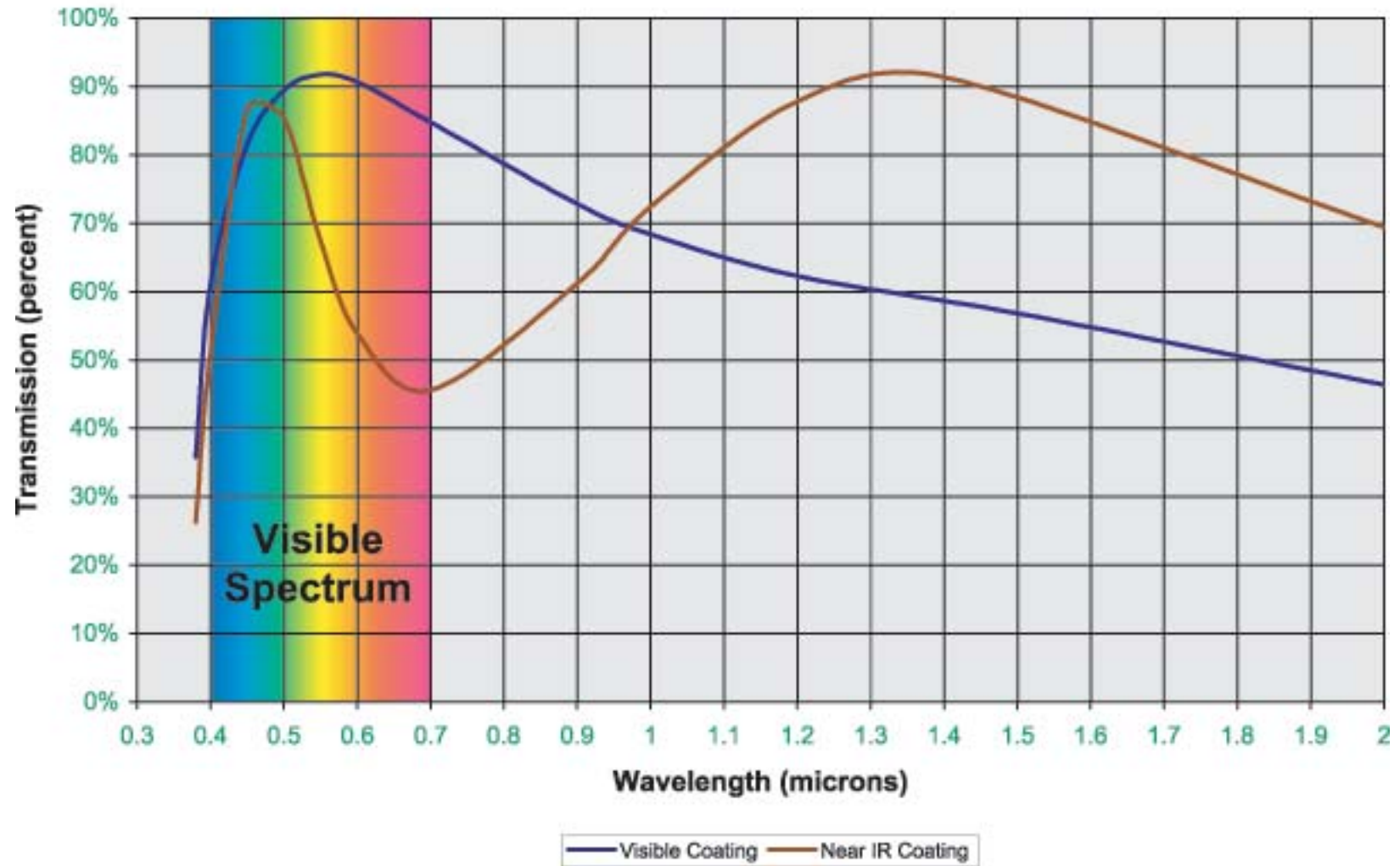
Transmission of the Zoom 6000 lens system
